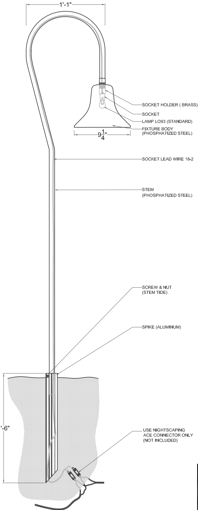
SIDE VIEW (HIDDEN) STANDARD MOUNTING
