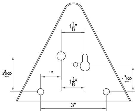
BACK VIEW
