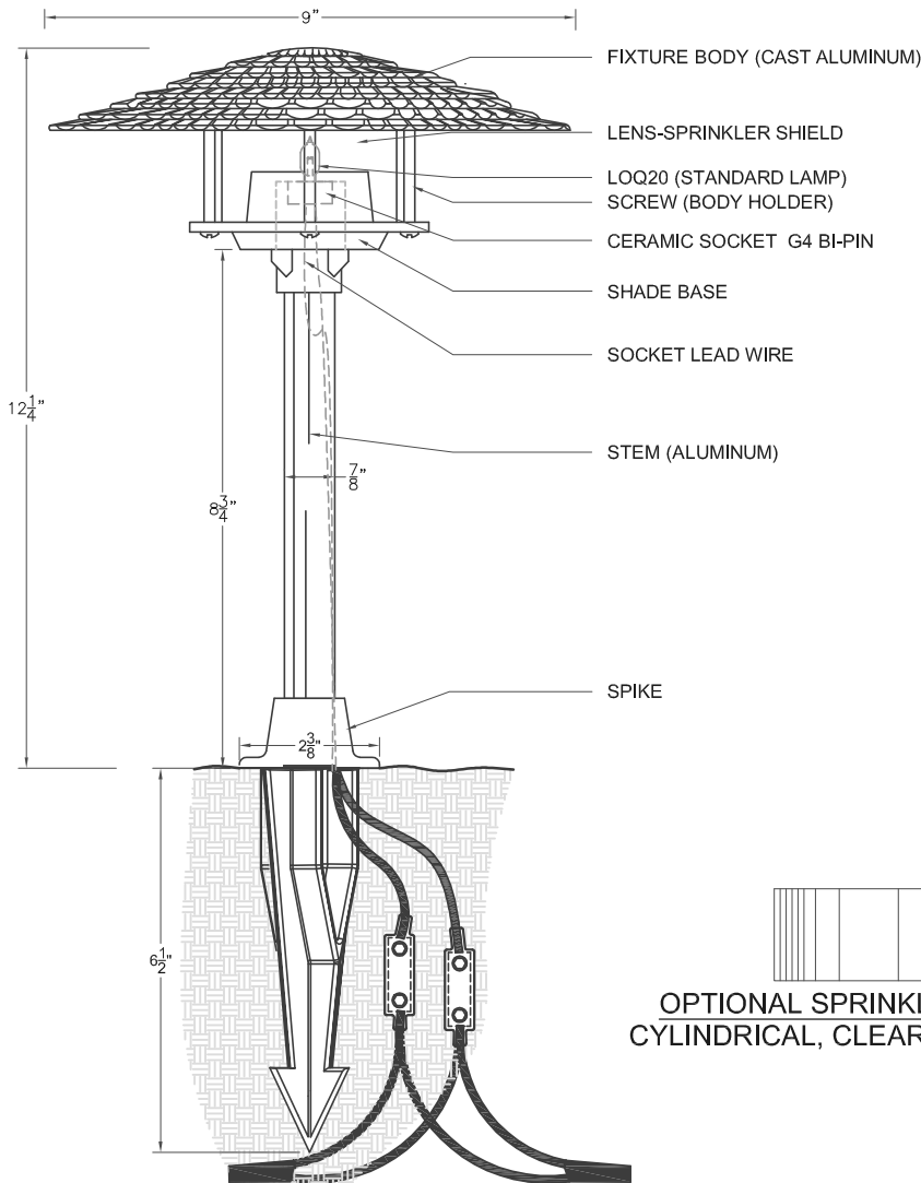
SIDE VIEW (HIDDEN)
