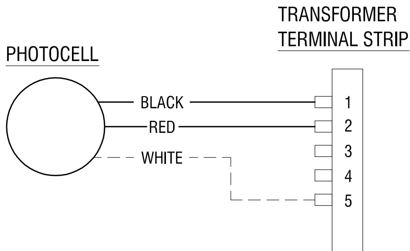
PC WIRING DIAGRAM
